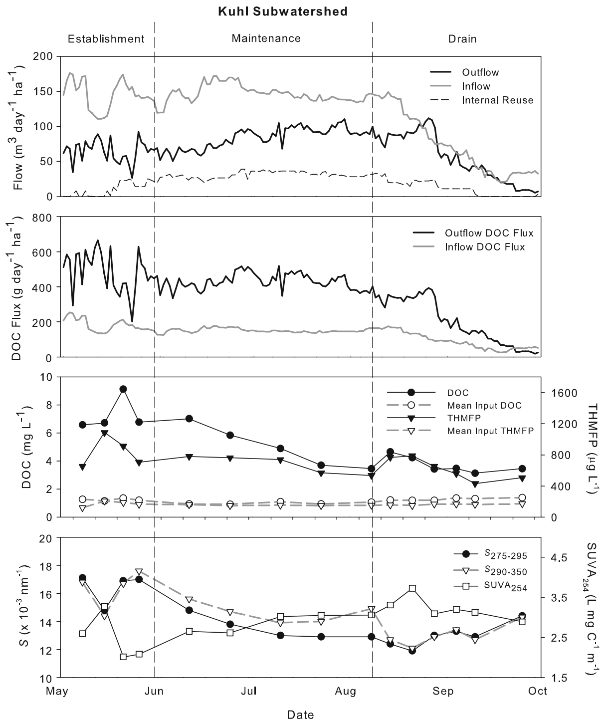
Fig. 3 Flow, internal reuse, DOC concentration and flux, THMFP, \text{SUVA}_{254} , and spectral slope ( S_{275-295} and S_{290-350} ) data obtained over the course of the growing season for the Kuhl subwatershed. Additionally, the average DOC and THMFP values of the three Main Canal sampling locations for each sampling event are included in the third panel. The
